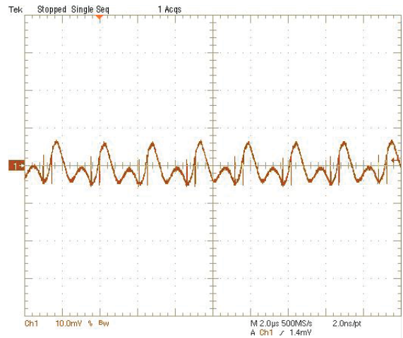
Output Ripple and Noise (Vin=12V, Vout=1.8V, Iout=20A, Cload=188µF, ScopeBW=20MHz) Trace1=Vout, 10mV/div(AC)
