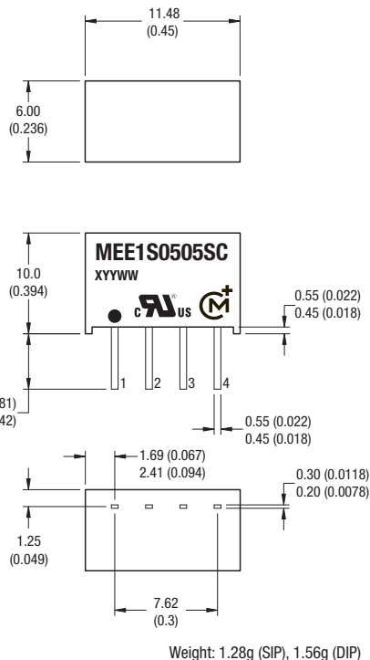
SIP Package
