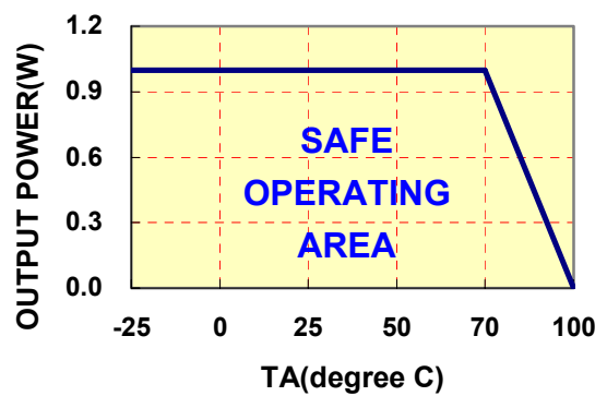
DERATING CURVE
