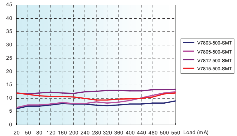
Output Voltage Ripple VS Output Load (Vin=Norm)
