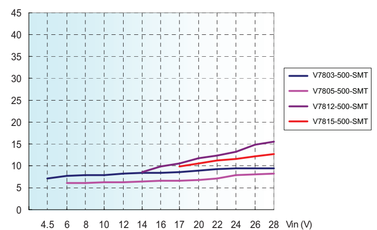
Output Voltage Ripple VS Input Voltage (Full Load)
