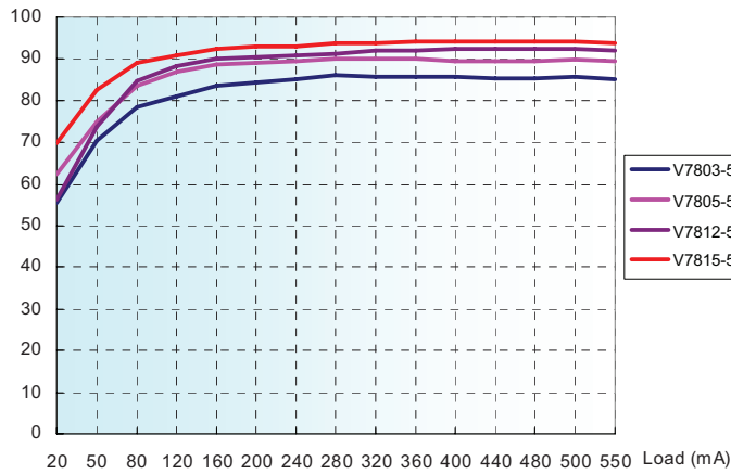
Efficiency VS Output Load (Vin=Norm)
