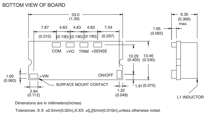
Figure 16 VPOL16A-12-SMT Mechanical Outline Diagram
