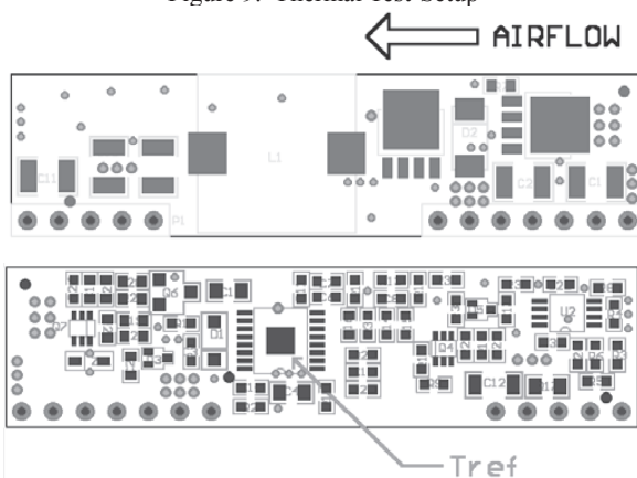
Figure 10. Temperature Measurement Location for VPOL16A-12W-SIP
