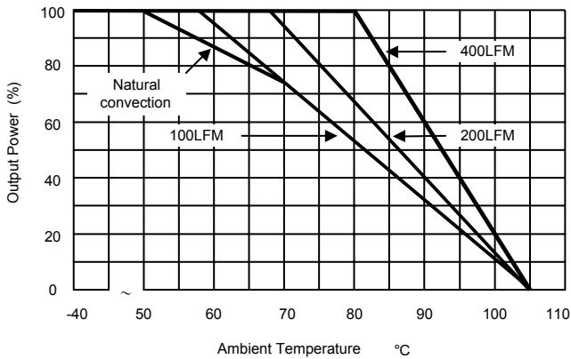
Derating Curve without Heatsink
